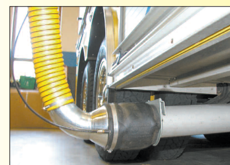
Virtually 100% Sealed Connection to Tailpipe
